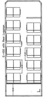
23 PASSENGER w/LUGGAGE
